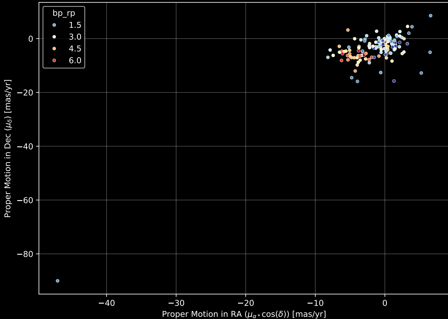
APOGEE DR17 Field: [008-02] Proper Motion Diagram (n= 137)
