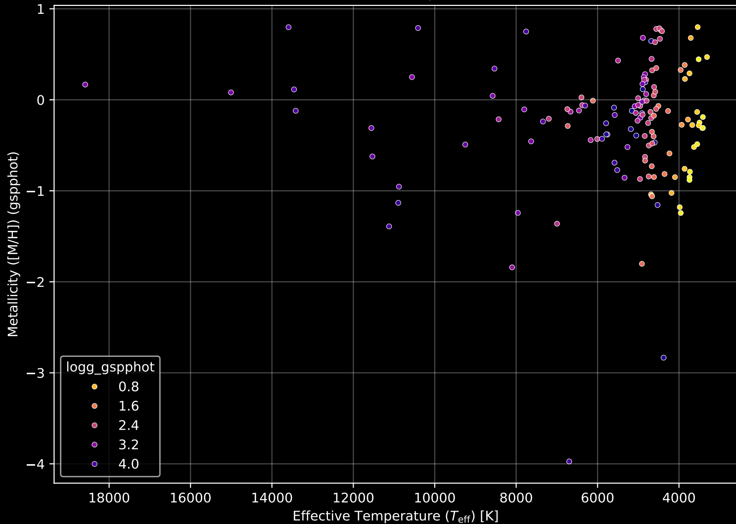
APOGEE DR17 Field: [008-02] Stellar Population Parameters (n= 137)
