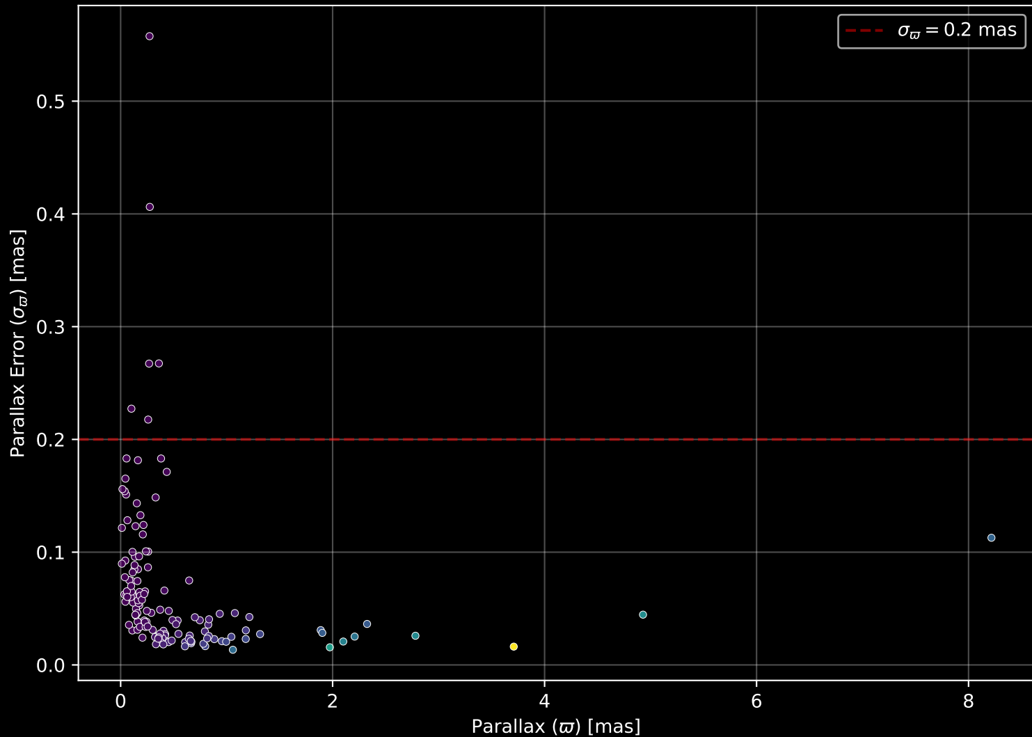
APOGEE DR17 Field: [008-02] Parallax Quality (n= 137)
