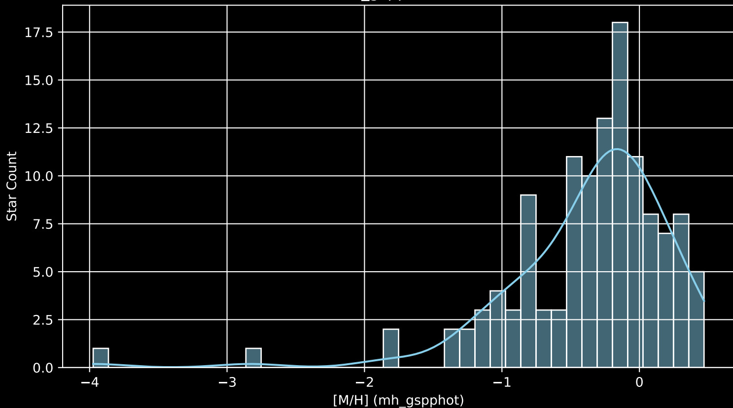
APOGEE DR17 Field: [008-02 [M/H] (mh_gspphot) (n= 124)
