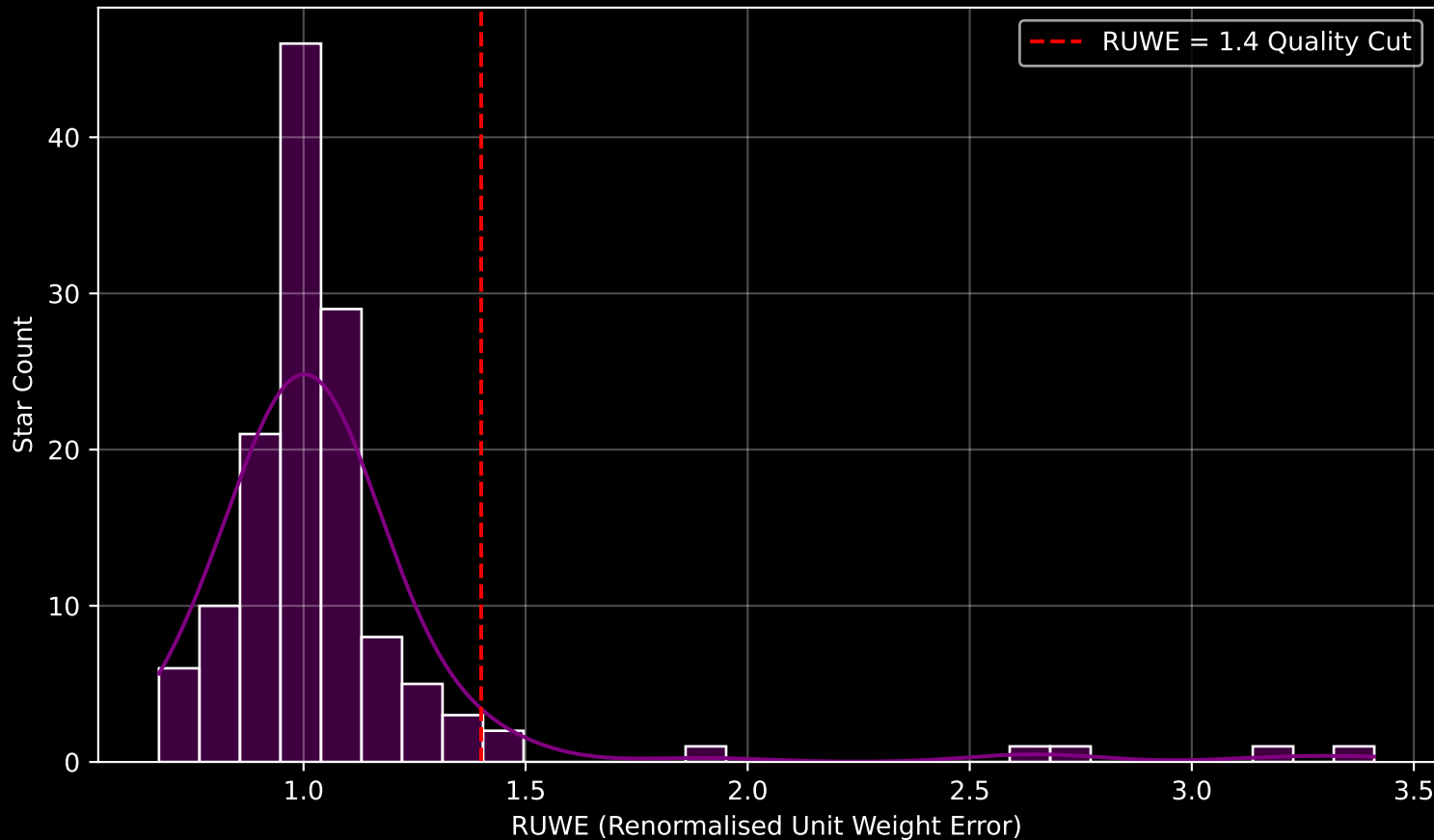
GAPOGEE DR17 Field [008-02] RUWE Distribution (n= 135)
